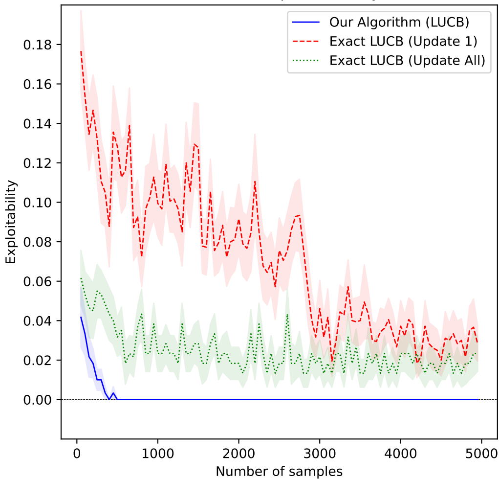
Kuhn Poker, Comparison, Player o
